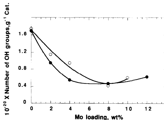
Fig. 3. The concentration of the surface OH groups as function of Mo content on various \text{MoO}_3/\text{TiO}_2 catalysts. ● Mo/anatase; ○ Mo/rutile.
