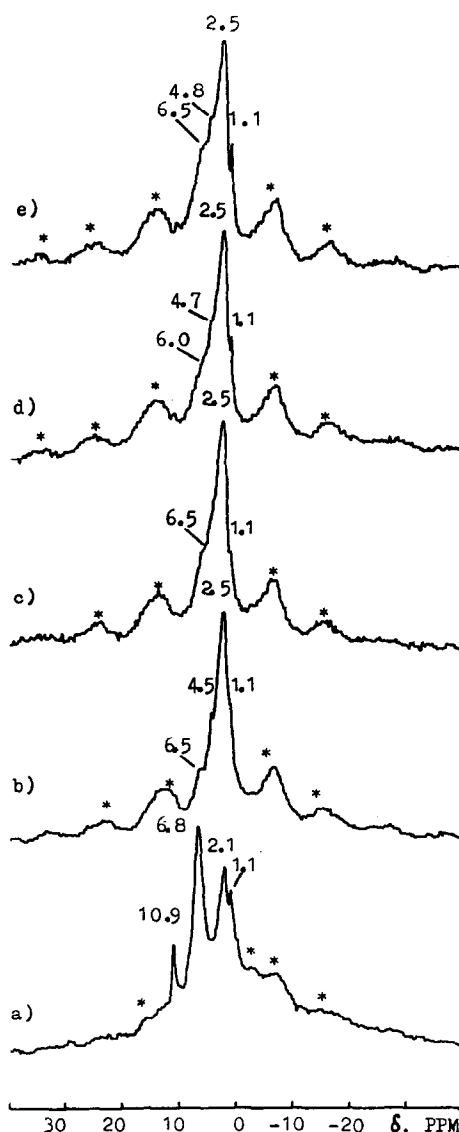
Fig. 1. ^1\text{H} NMR MAS spectra of \text{TiO}_2 (anatase) and \text{MoO}_3/\text{TiO}_2 (anatase) samples at various 'Mo' levels. (a) \text{TiO}_2 (anatase); (b) 2% Mo; (c) 4% Mo; (d) 8% Mo; (e) 12% Mo.
