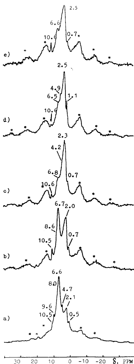
Fig. 2. ^1\text{H} NMR MAS spectra of \text{TiO}_2 (rutile) and \text{MoO}_3/\text{TiO}_2 (rutile) samples at various 'Mo' levels. (a) \text{TiO}_2 (rutile); (b) 2% Mo; (c) 4% Mo; (d) 8% Mo; (e) 10% Mo.
